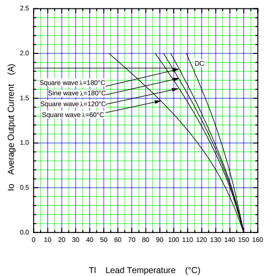
Current Derating ( I_O - T_L )
