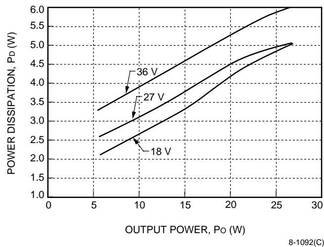
Figure 24. CC025ACL-M Fixed Losses, P_p
