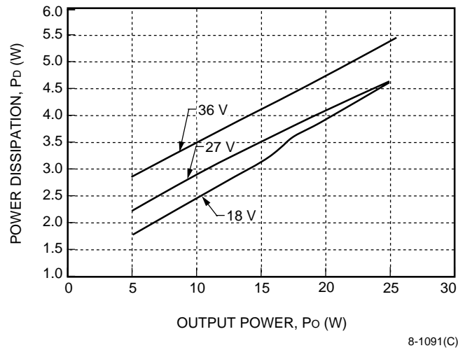
Figure 23. CC025ABK-M Fixed Losses, P_p
