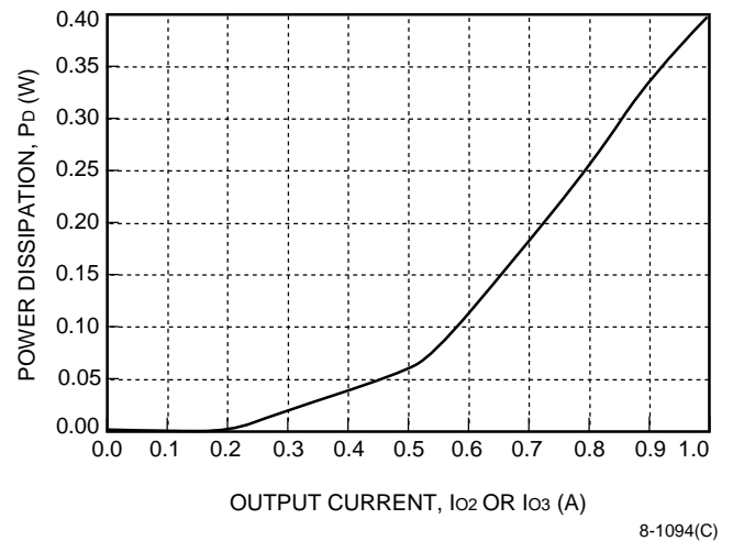
Figure 26. CC025ABK-M, Losses Associated with \pm 12 V Output, P_{s2}/P_{s3}
