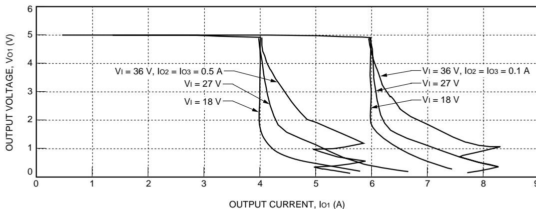
Figure 9. CC025ABK-M Typical 5 V Output Characteristics
