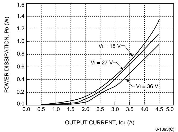
Figure 25. CC025ABK-M, CC025ACL-M Losses, Associated with 5 V Output, P_{s1}
