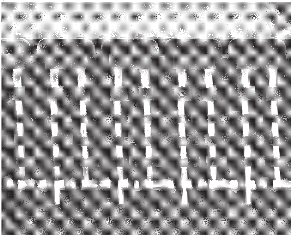
Figure 3. HCMOS7 Back end Cross Section
