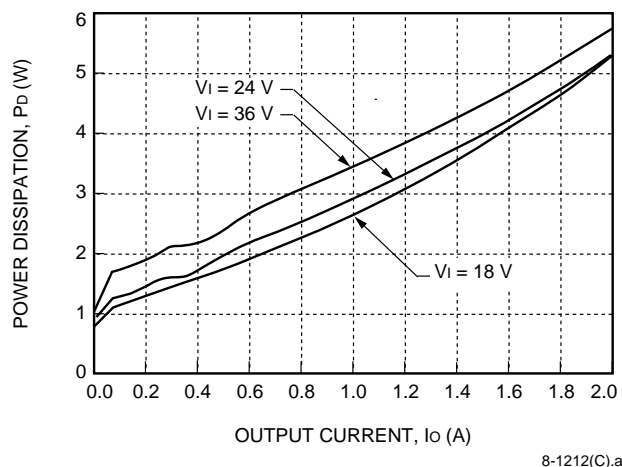
Figure 23. CC030C Power Dissipation vs. Output Current
