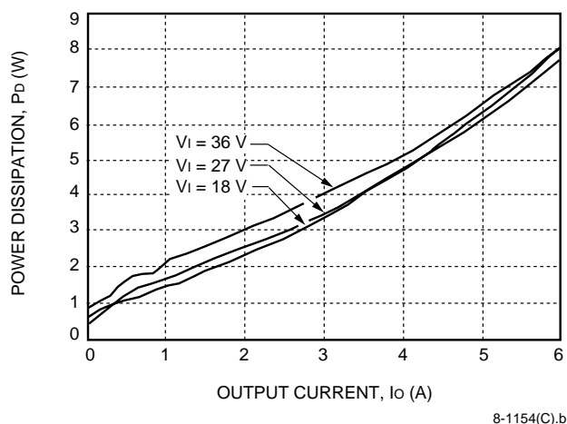
Figure 21. CC030A Power Dissipation vs. Output Current
