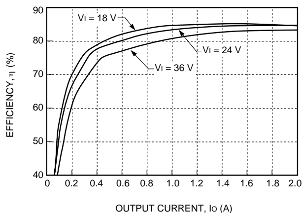
Figure 10. CC030C Typical Converter Efficiency vs. Output Current
