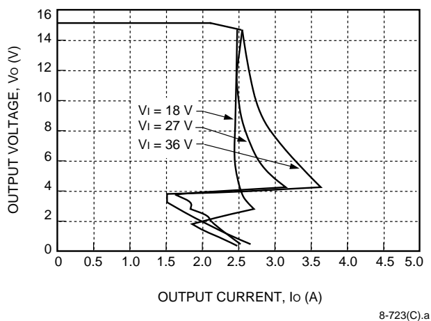
Figure 4. CC030C Typical Output Characteristics
