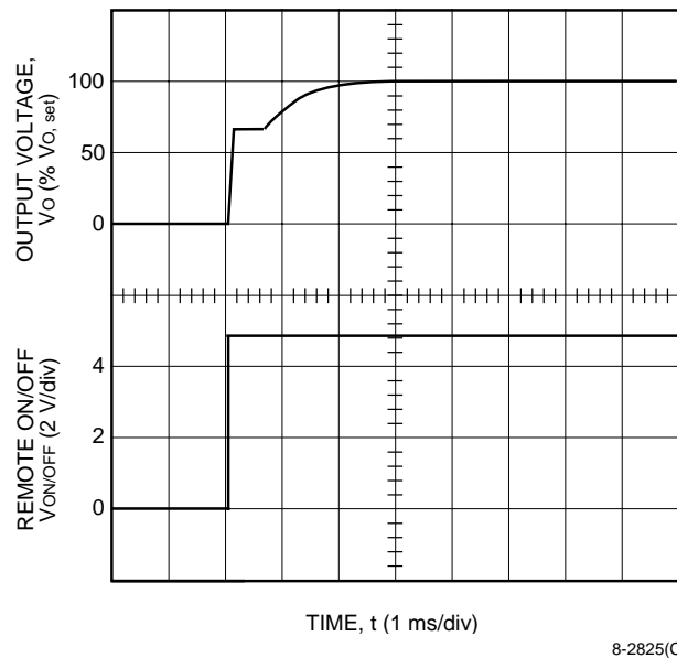
Figure 13. Typical Output Voltage Start-Up when Signal Applied to Remote On/Off
