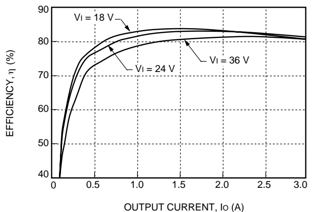
Figure 9. CC030B Typical Converter Efficiency vs. Output Current
