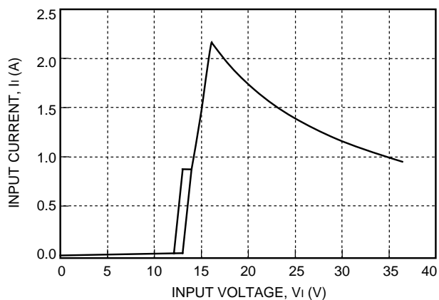
Figure 1. CC030-Series Typical Input Characteristic
