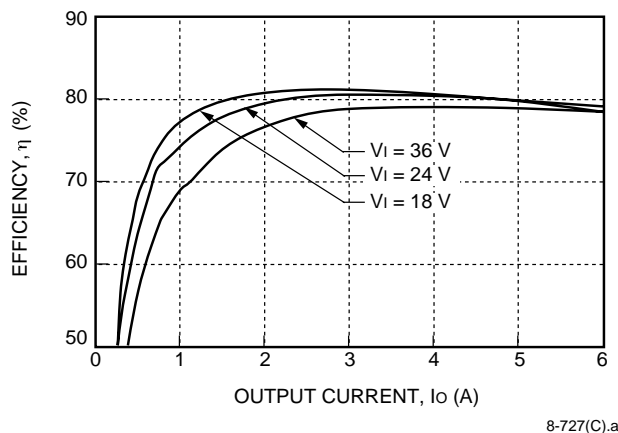
Figure 8. CC030A Typical Converter Efficiency vs. Output Current
