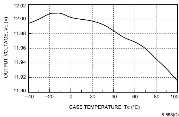
Figure 6. CC030B Typical Output Voltage Variation over Ambient Temperature Range
