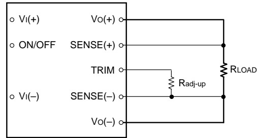
Figure 18. Circuit Configuration to Increase Output Voltage
