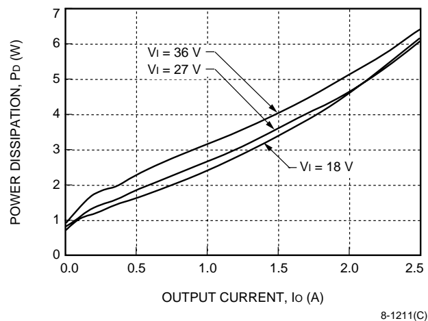
Figure 22. CC030B Power Dissipation vs. Output Current
