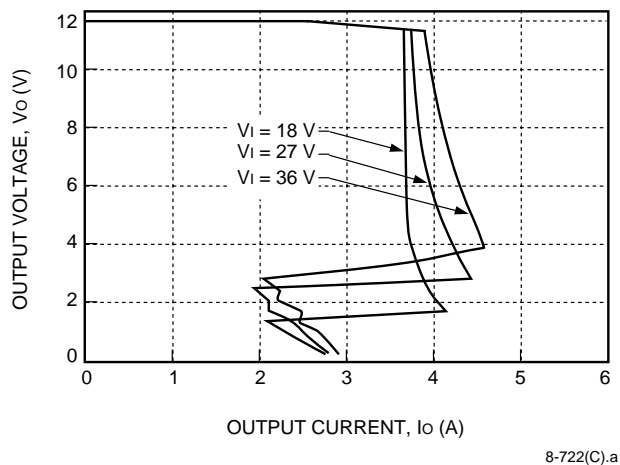
Figure 3. CC030B Typical Output Characteristics
