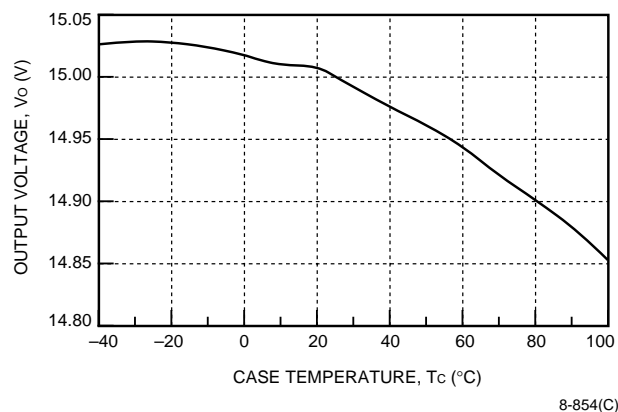
Figure 7. CC030C Typical Output Voltage Variation over Ambient Temperature Range
