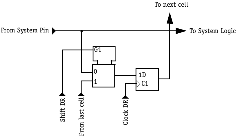
Figure 7 Observe-Only Cell
