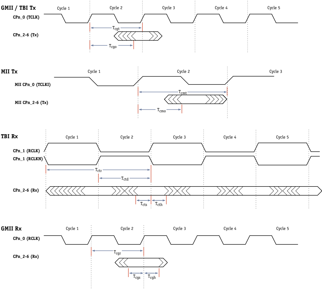
Figure 14 Gigabit Ethernet and TBI Interface Timing Diagram
