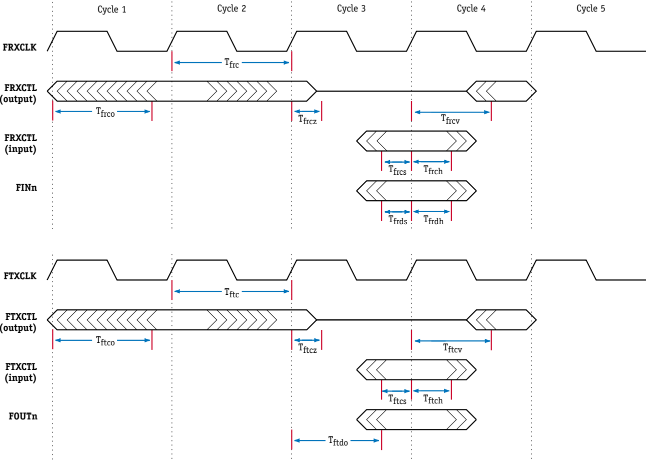
Figure 21 Fabric Processor Timing Diagram
