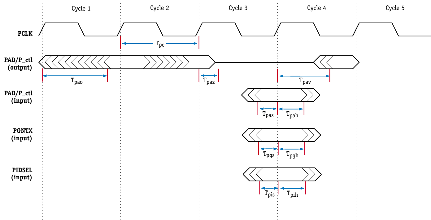
Figure 17 PCI Timing Diagram
