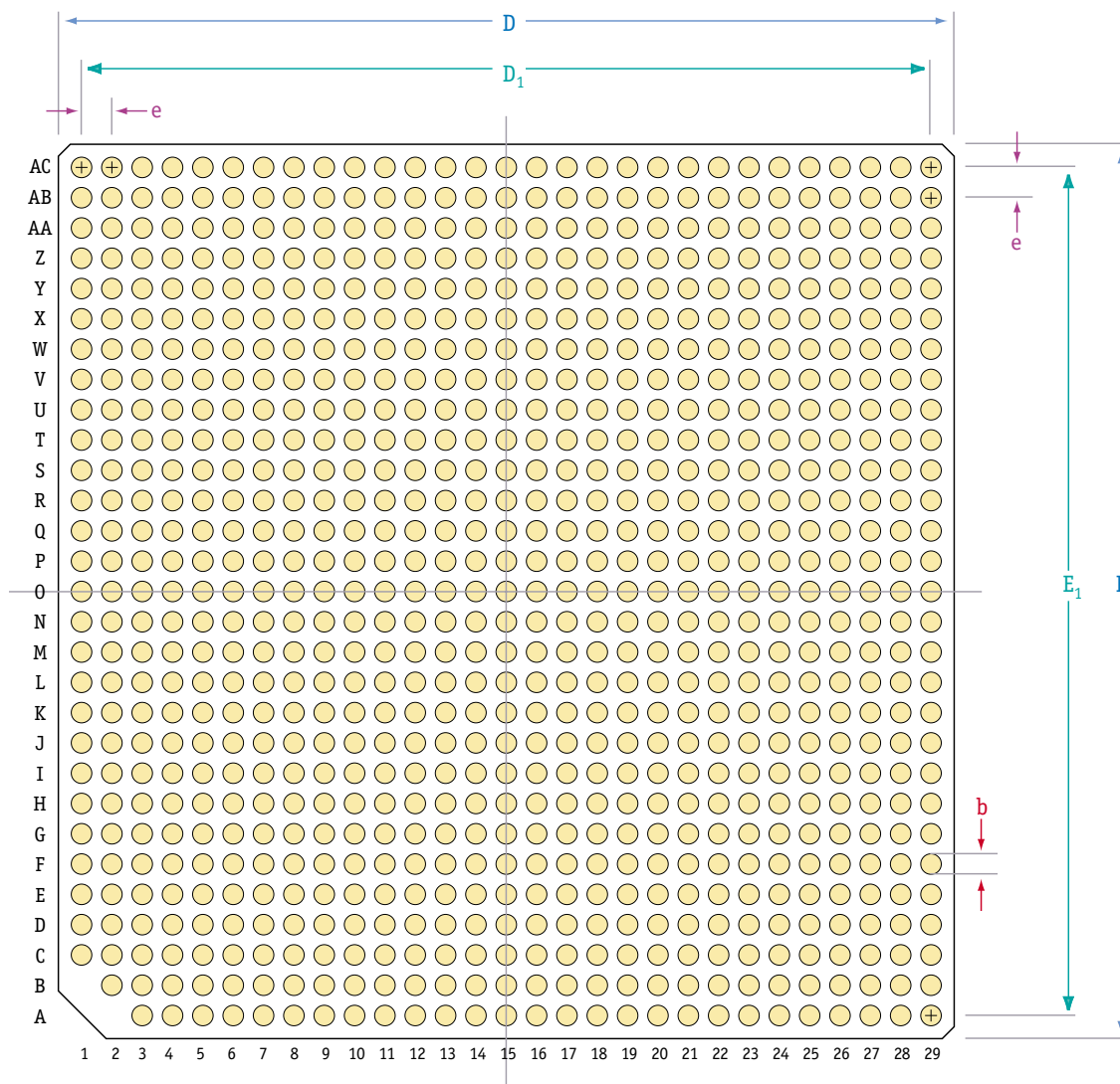
Figure 26 C-5 Network Processor BGA Package (Bottom View)
