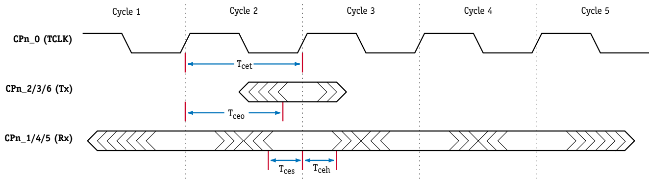
Figure 13 10/100 Ethernet Timing Diagram
