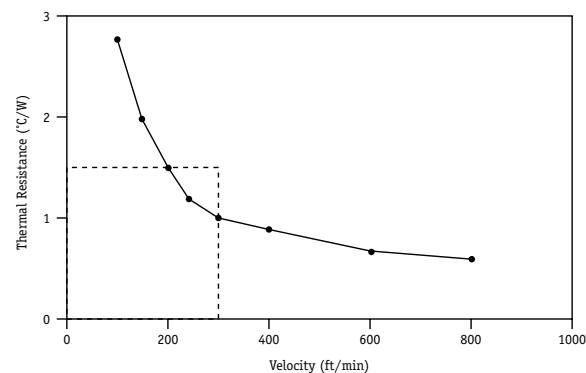
Figure 10 Thermal Performance for C-5 Network Processor Heat Sink (see step 2 above)
