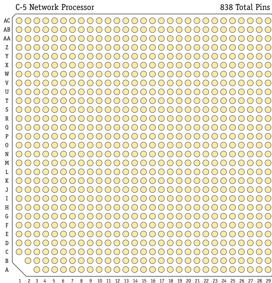
Figure 2 Pin Locations (Bottom View)
