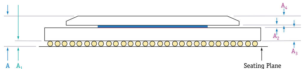
Figure 25 C-5 Network Processor BGA Package Side View
