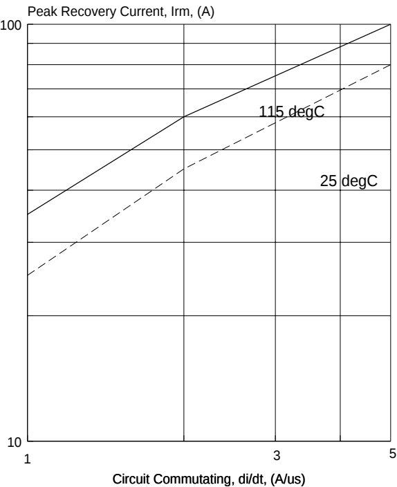
MAXIMUM PEAK RECOVERY CURRENT versus COMMUTATING di/dt
