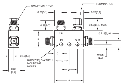
SERIES CA OUTLINES 1-8
