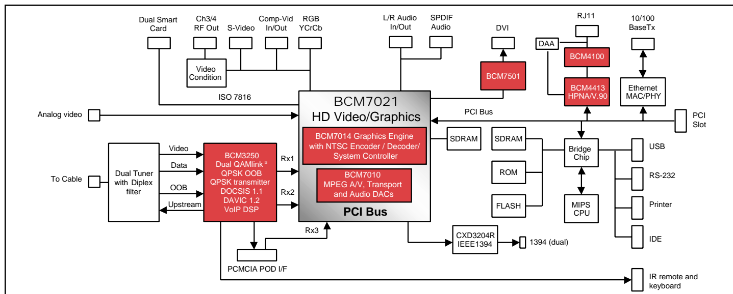
BCM7021 Advanced Video, Graphics, and Audio Subsystem
