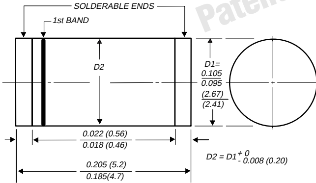
DO-213AB
