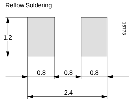
Figure 6. Recommended foot pads (in mm)
