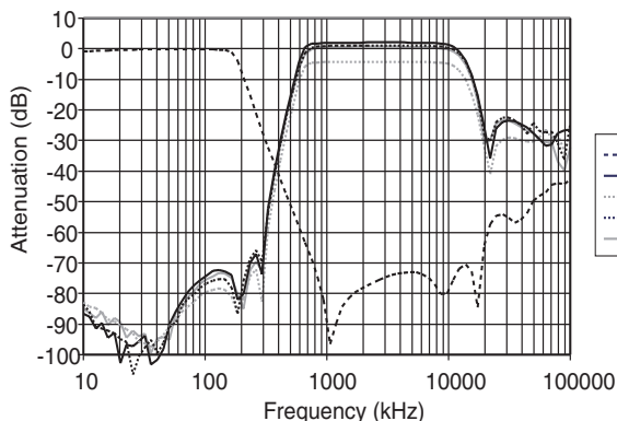
B4010/11/14 Frequency Response
