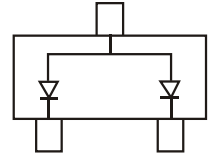
BAS70-06 Marking: K76, K7F
