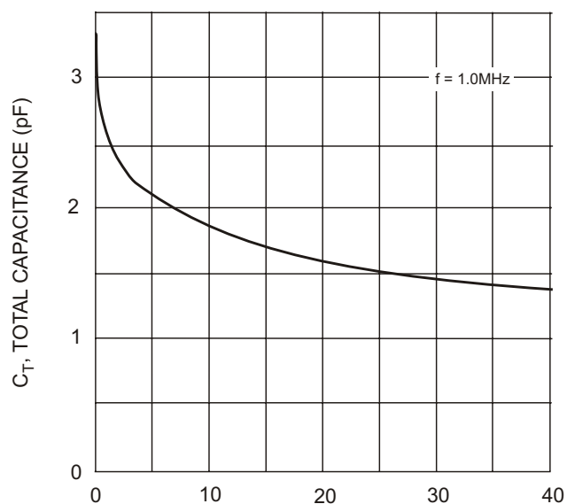
Fig. 3 Typical Capacitance
