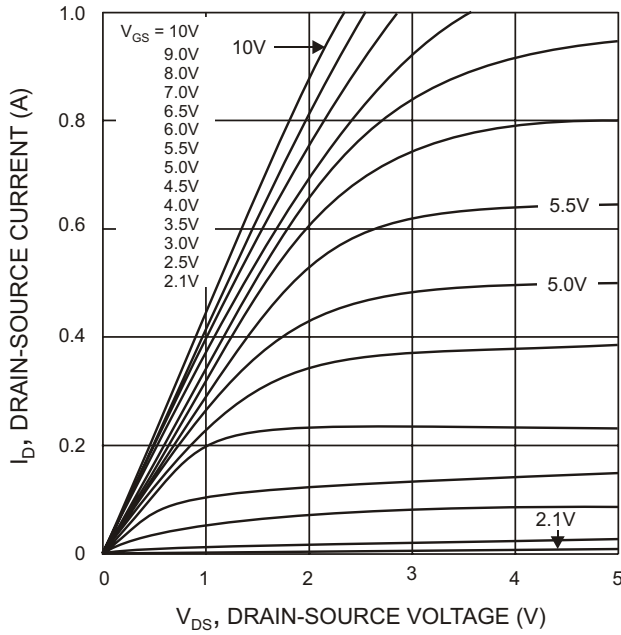
Fig. 1 On-Region Characteristics
