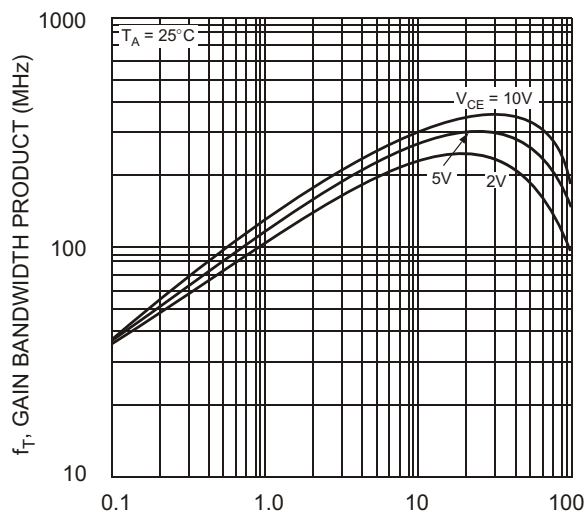
Fig. 4, Gain Bandwidth Product vs Collector Current (BC847B)
