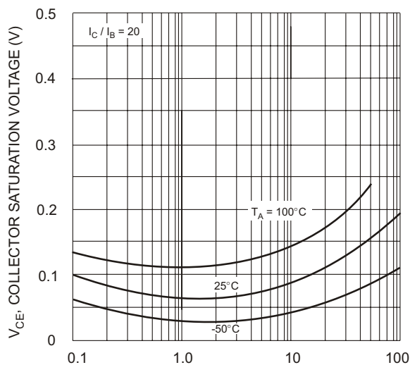
Fig. 3, Collector Saturation Voltage vs Collector Current (BC847B)
