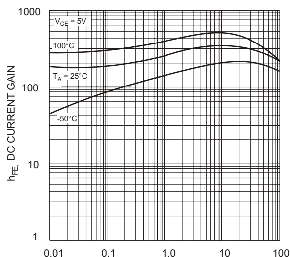
Fig. 2, DC Current Gain vs Collector Current (BC847B)
