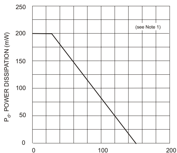
Fig. 1, Power Derating Curve (Total Device)
