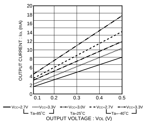
Fig.20 V_{OL} - I_{OL} features (Note : Typ.)
