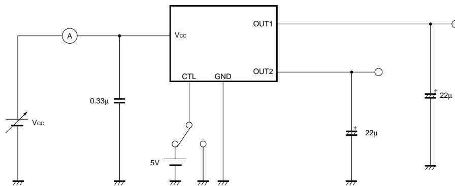
Fig.3 Circuit for measuring minimum I/O voltage difference
