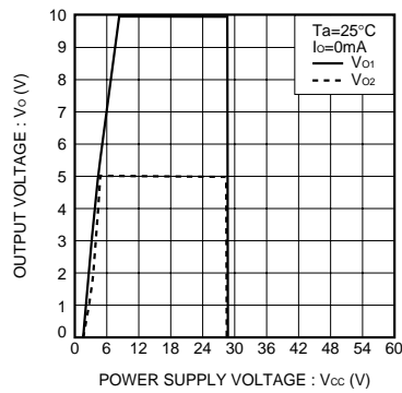
Fig.11 Output voltage characteristic (Typ.)
