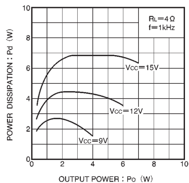
Fig. 14 Power dissipation vs. output power (II)
