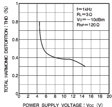
Fig. 8 Distortion vs. power supply voltage
