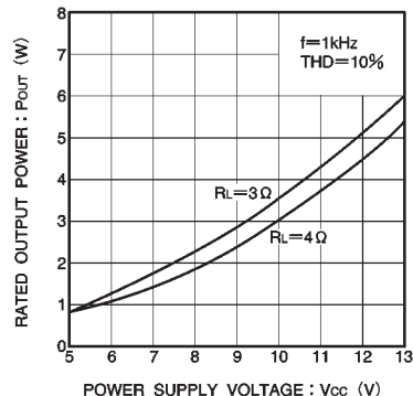
Fig. 11 Output power vs. power supply voltage
