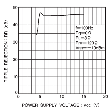
Fig. 17 Ripple rejection ratio vs. power supply voltage
