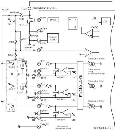
Example of R.G.B flash LED
