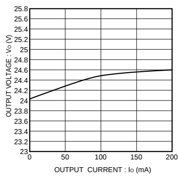
Fig.13 Load regulation
