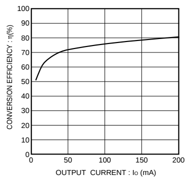
Fig.15 Conversion efficiency
