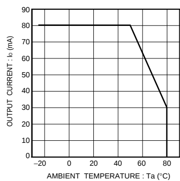
Fig.15 Derating curve
