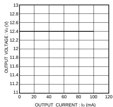
Fig.13 Output characteristic
