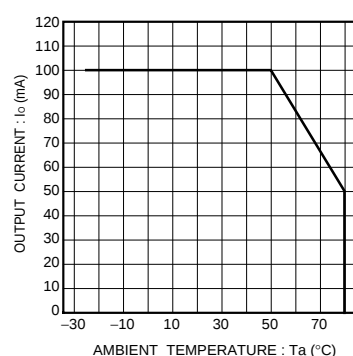
Fig.7 Derating curve
