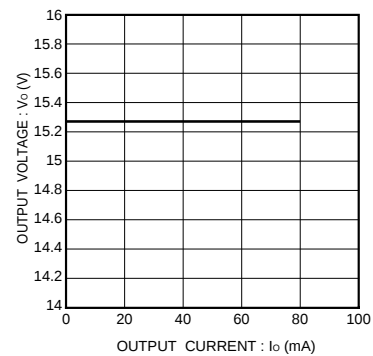
Fig.17 Output characteristic
