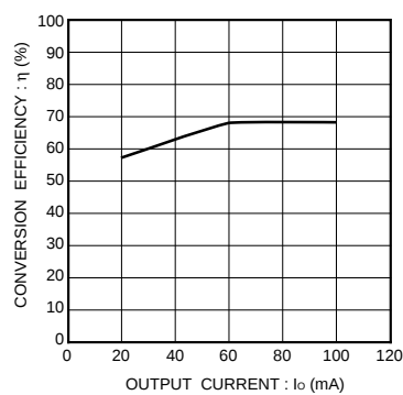
Fig.14 Conversion efficiency
