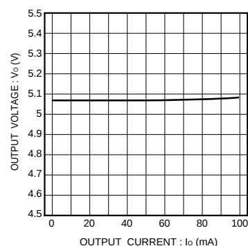
Fig.9 Output characteristic
