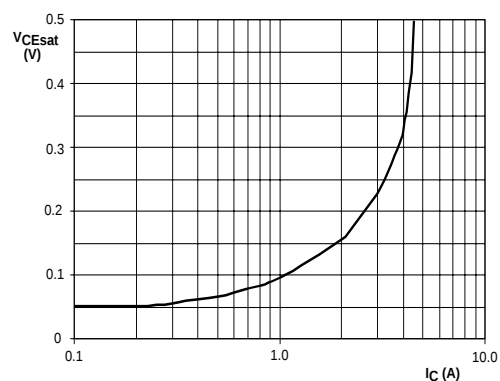
Fig.11. Collector-Emitter saturation voltage. Solid lines = typ values, V_{CEsat} = f(I_C) ; at I_C/I_B = 4 .
