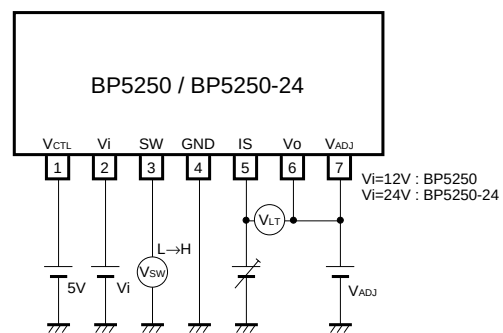
Over current detection off set voltage 1 : V_{ADJ}=1.25V Over current detection off set voltage 2 : V_{ADJ}=0V Fig.2 Over current detection off set voltage measurement circuit
