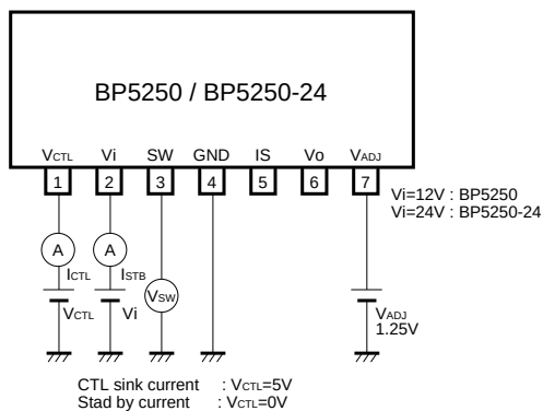
CTL sink current : V_{CTL}=5V Stand by current : V_{CTL}=0V Fig.3 Control terminal voltage sink current · Stand by sink current measurement circuit
