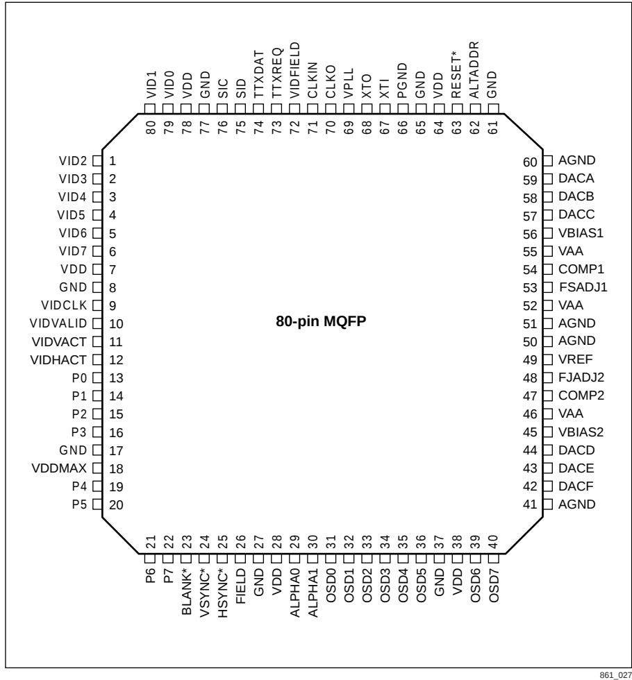
Figure 1-1. Pinout Diagram
