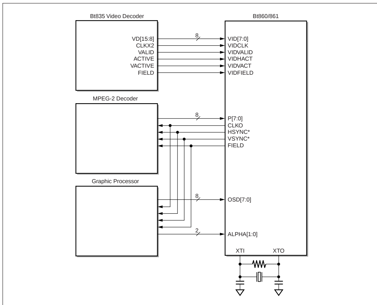
Figure 2-9. Video Decoder Connection Example
