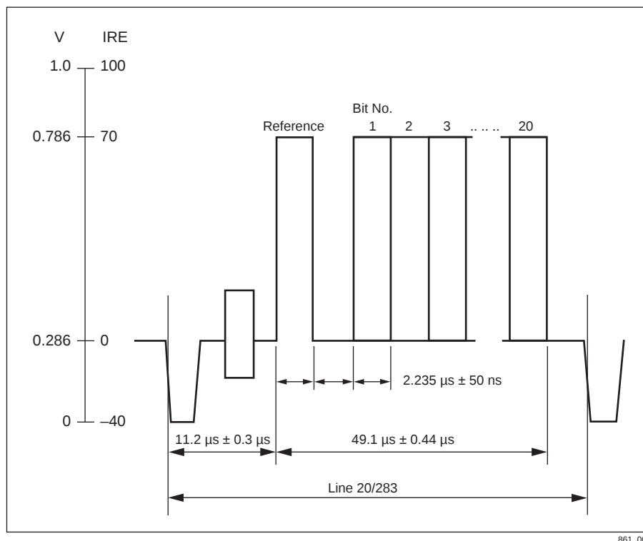
Figure 3-19. CGMS Waveform
