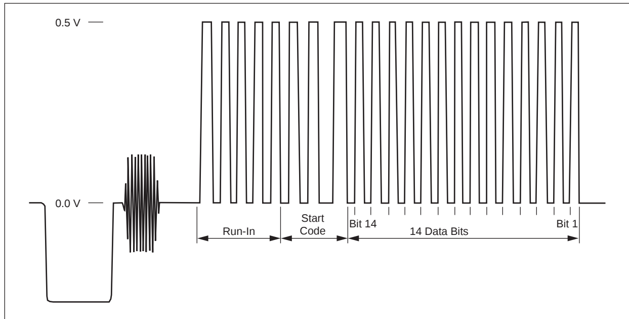
Figure 3-18. WSS Waveform
