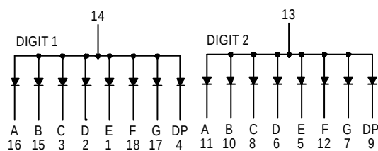
(BVN-2502 Common Anode.)
