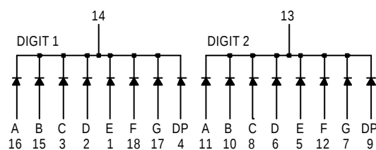
(BVN-7502 Common Cathode.)
