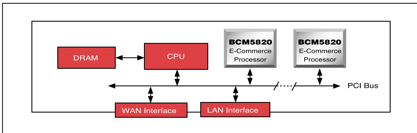
SSL/TLS E-Commerce Server Diagram
