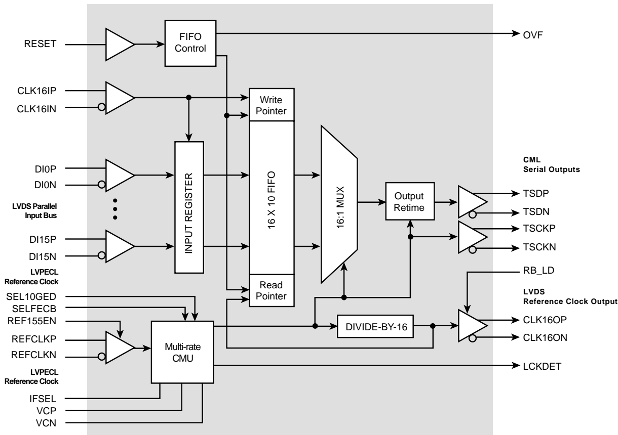
Block Diagram
