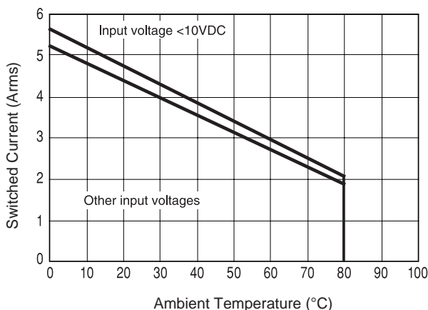
Figure 4 – Thermal curves
