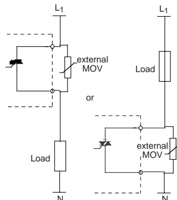
Figure 3 – BS relays
