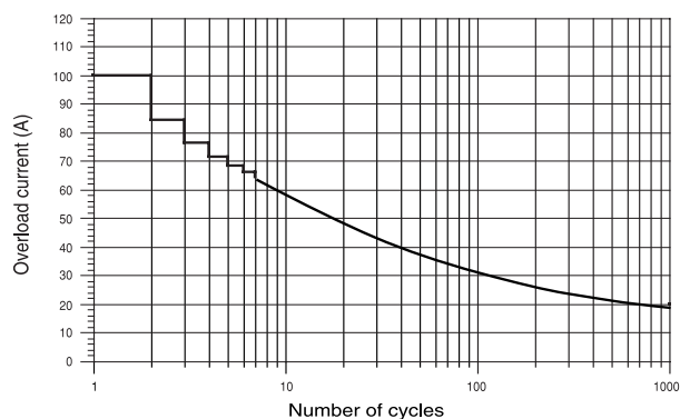
Figure 5 – Non-repetitive surge current
