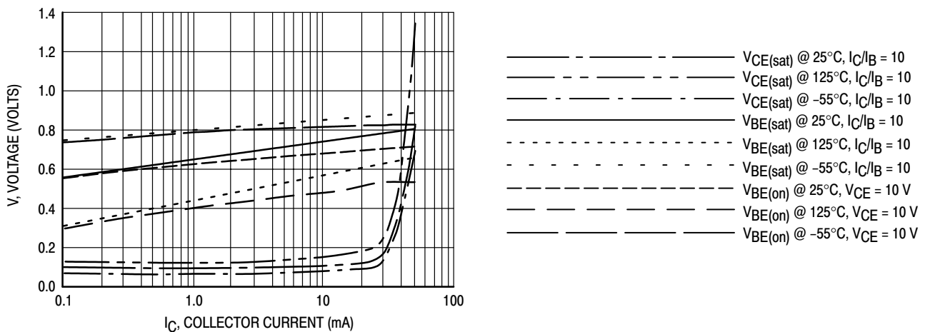
Figure 4. "ON" Voltages
