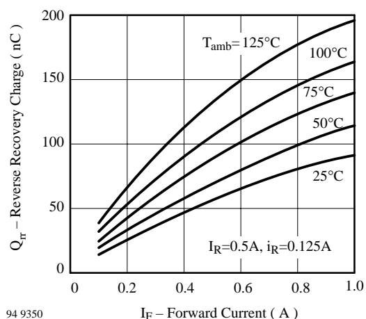
Figure 6. Max. Reverse Recovery Charge vs. Forward Current
