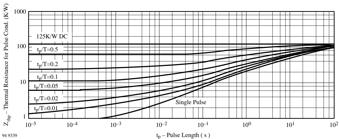
Figure 7. Thermal Response
