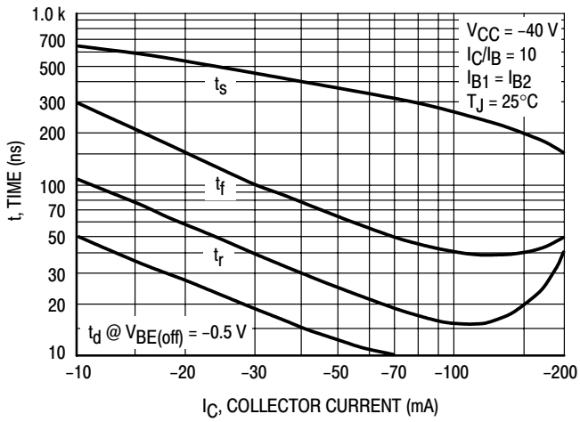
Figure 3. Switching Times
