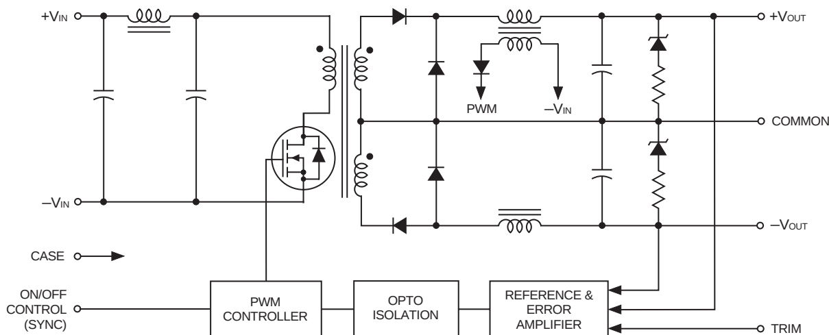
Figure 1. Simplified Schematic
