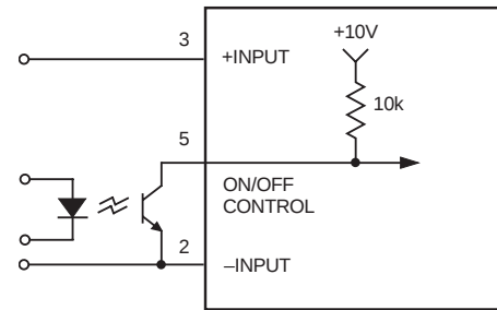
Figure 6. Driving the On/Off Control Pin
