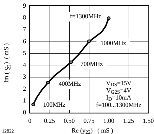
Figure 11. Short Circuit Output Admittance
