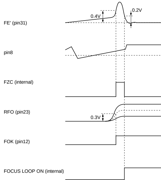
Fig.4 LOOP ON timing
