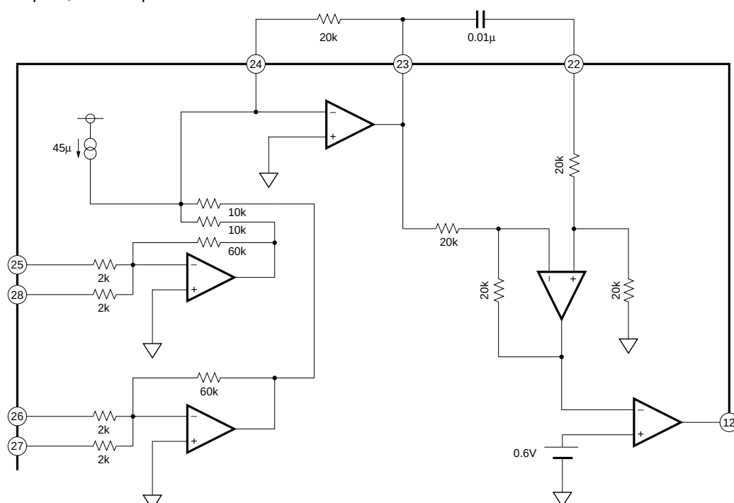
Fig.2 RF and FOK block
