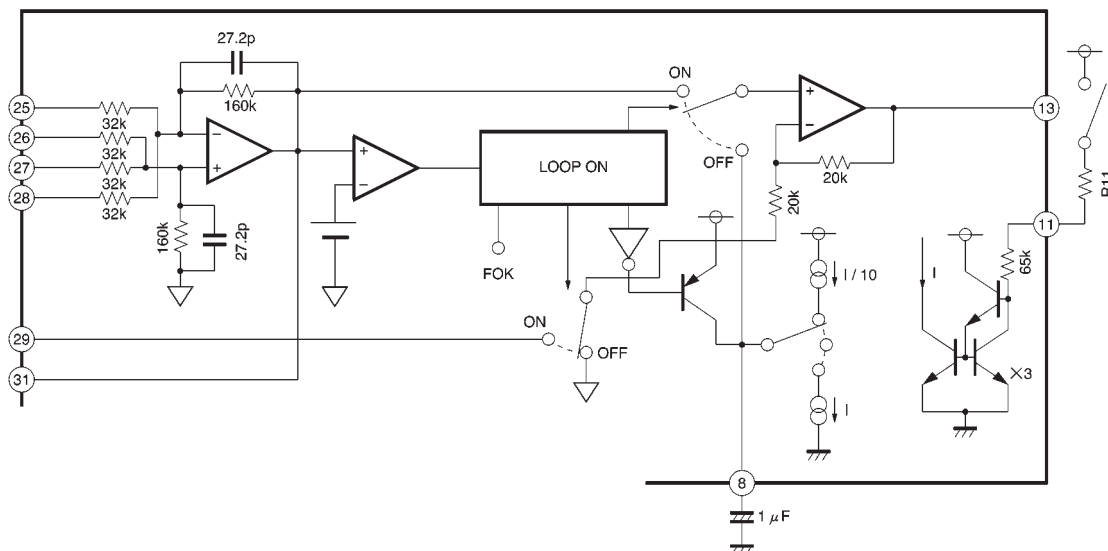
Fig.3 Focus error block
