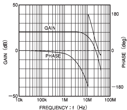
Fig.10 RF amplifier frequency characteristics
