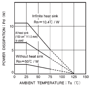
Fig.4 Thermal derating
