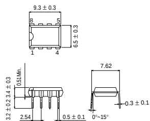
DIP8
