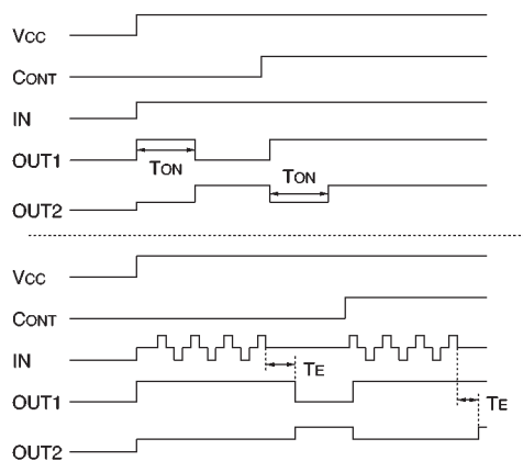
●Timing chart
