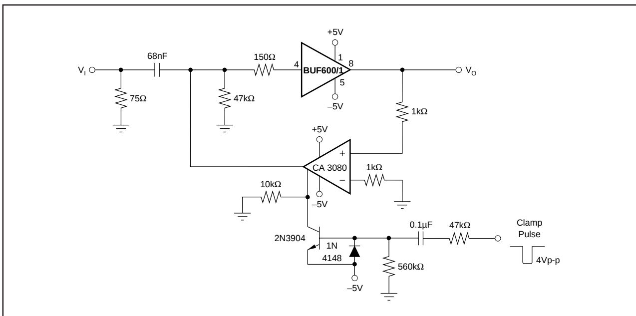
FIGURE 8. Input Amplifier with Baseband Video DC Restoration.
