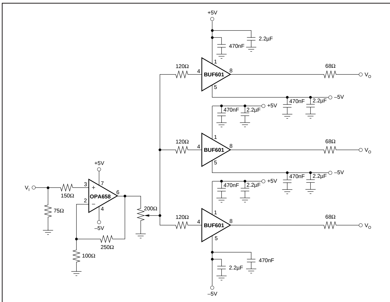
FIGURE 5. Video Distribution Amplifier.
