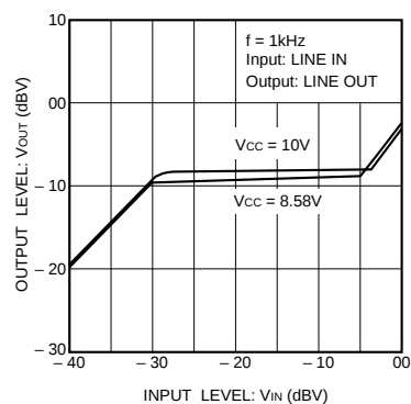
Fig. 8 ALC input / output characteristics
