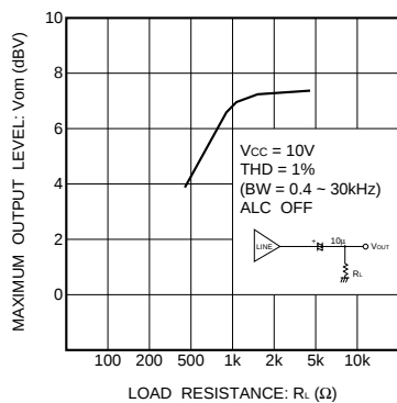
Fig. 7 Line amplifier load drive characteristics
