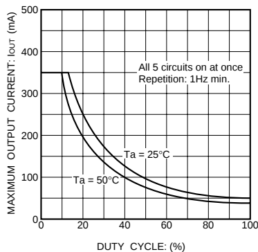
Fig.3 Output current vs. duty cycle
