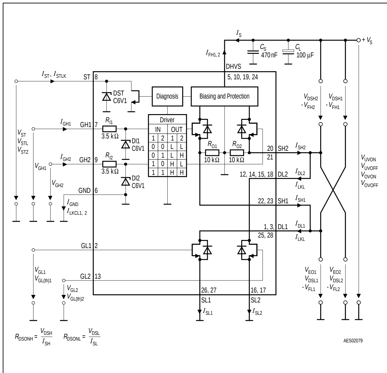
Figure 3 Test Circuit
