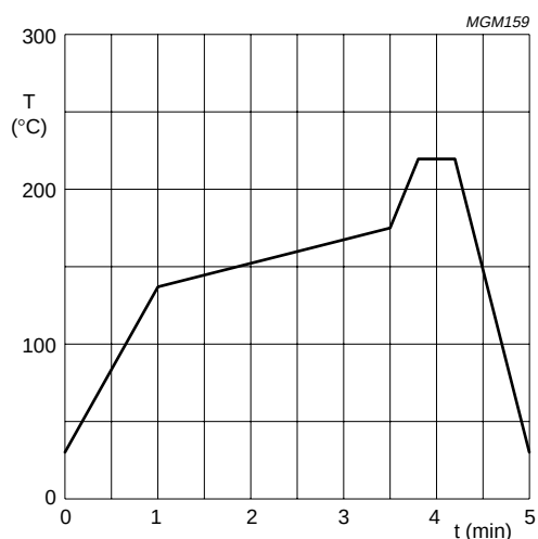
Fig.17 Recommended reflow temperature profile.
