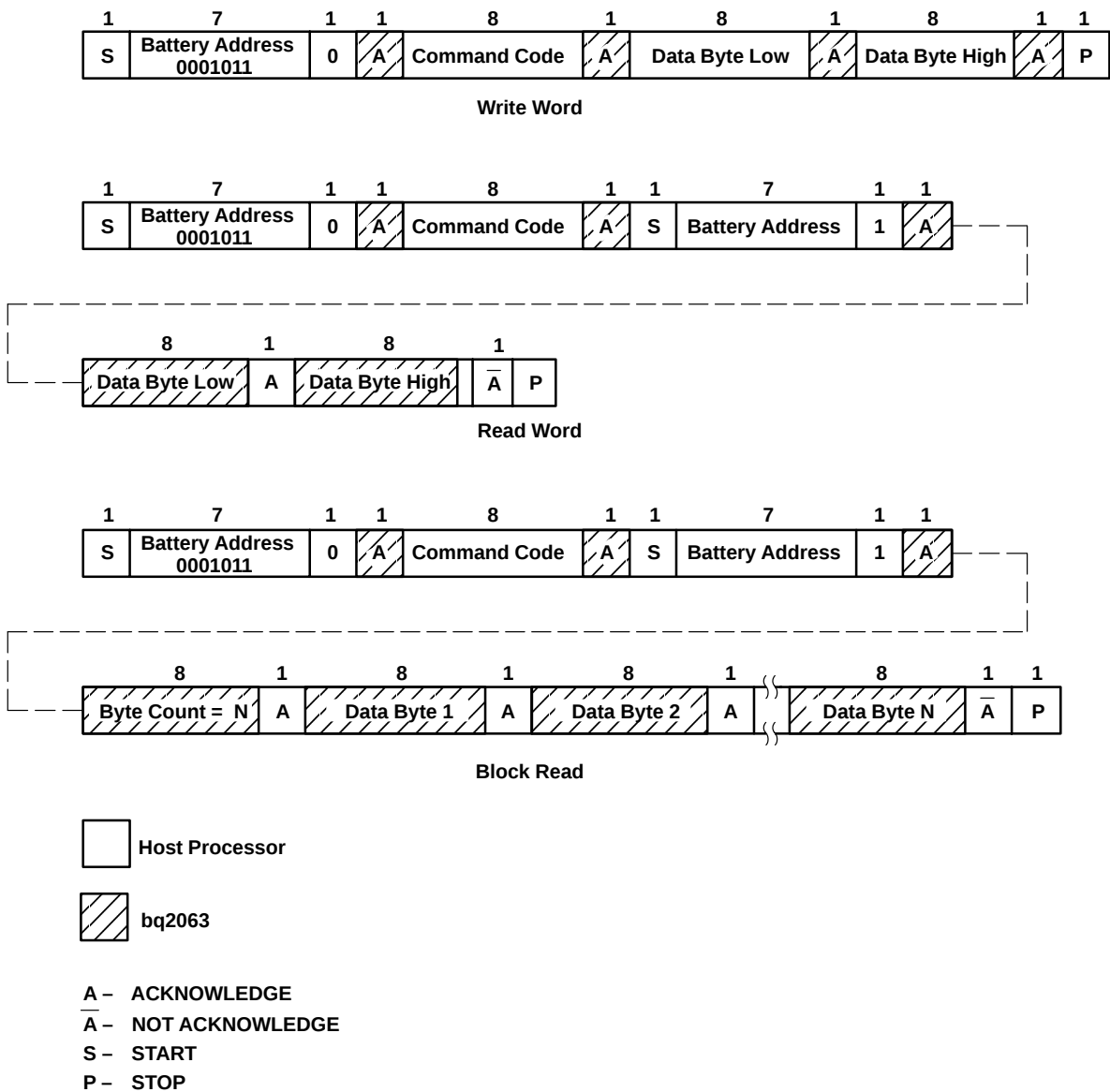
Figure 8. SMBus Communication Protocol Without PEC
