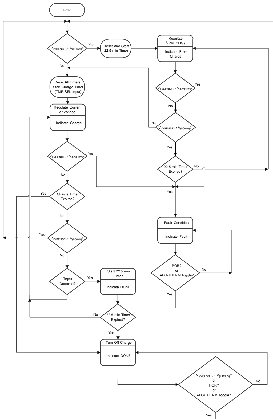
Figure 14. Operational Flow Chart With the Charge Termination Timers Enabled ( \overline{\text{TMR EN}} = 0 )
