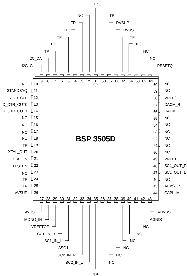
Fig. 5–6: 68-pin PLC package
