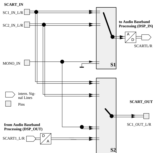
Fig. 2–1: SCART-Switching Facilities (see 4.4.12.) positions show the default configuration after Power On Reset.
