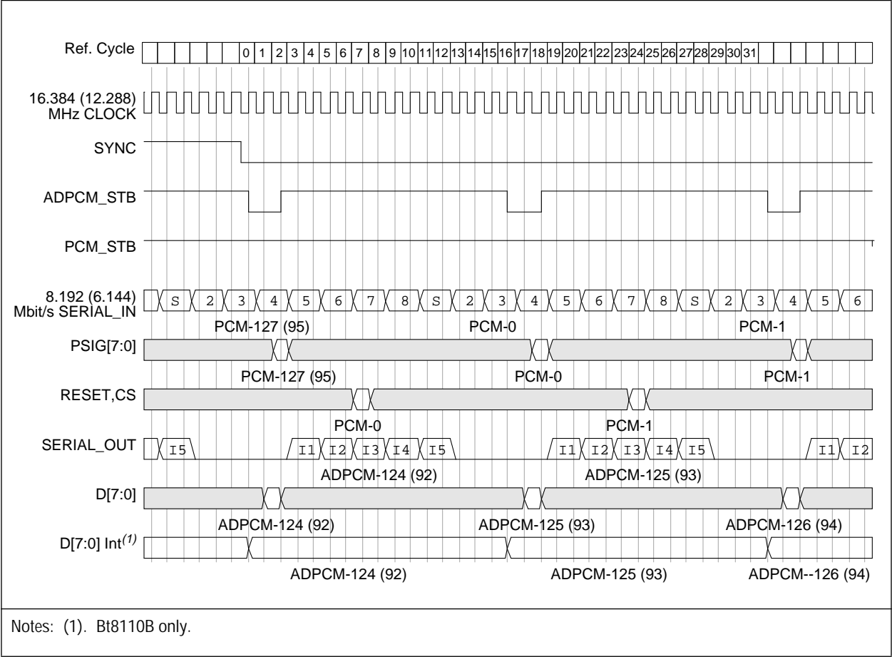
Figure A-3. 96- or 128-Channel Half-Duplex Encoder-Only Functional Timing
