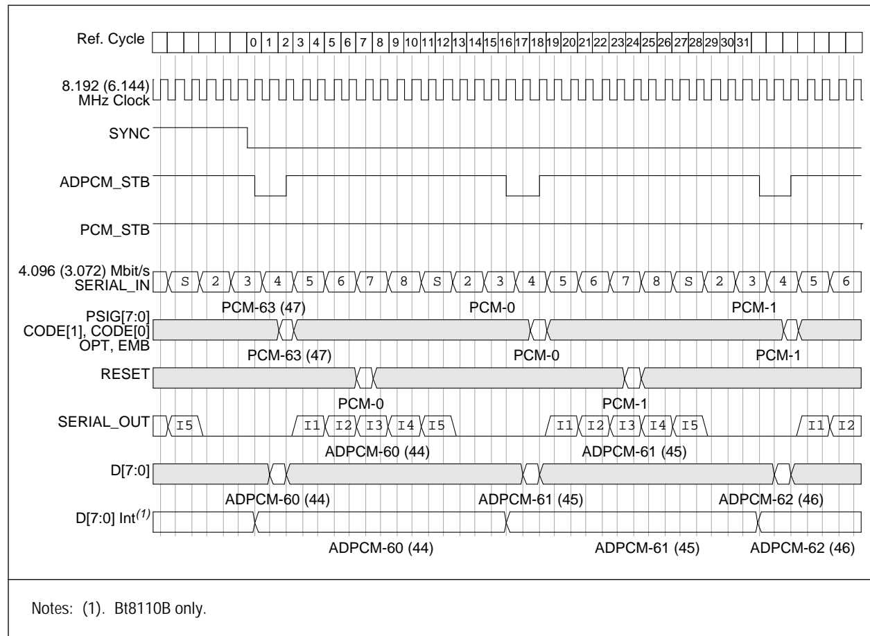
Figure 2-7. Hardware Control Encoder-Only Timing
