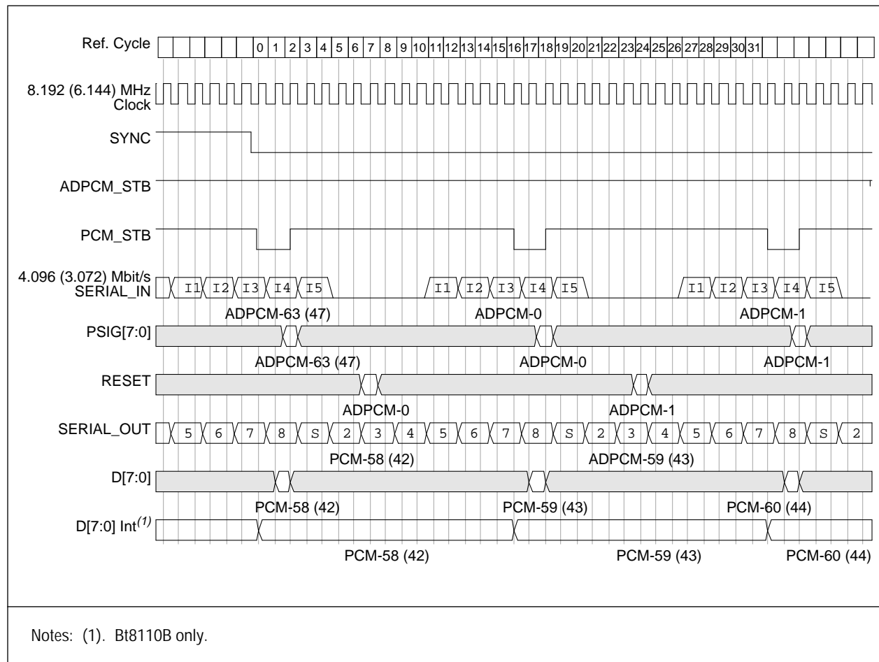
Figure 2-5. Input and Output Timing for 48- or 64-Channel Half-Duplex Decoder-Only Operation (Microprocessor Control)
