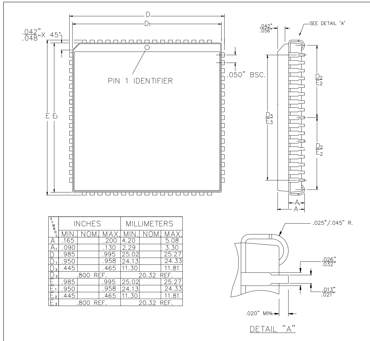
Figure 4-3. 68-Pin Plastic Leaded Chip Carrier (J-Bend)
