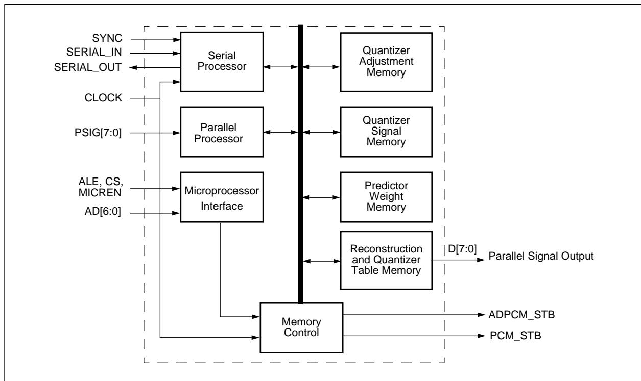
Figure 2-2. Bt8110B Block Diagram
