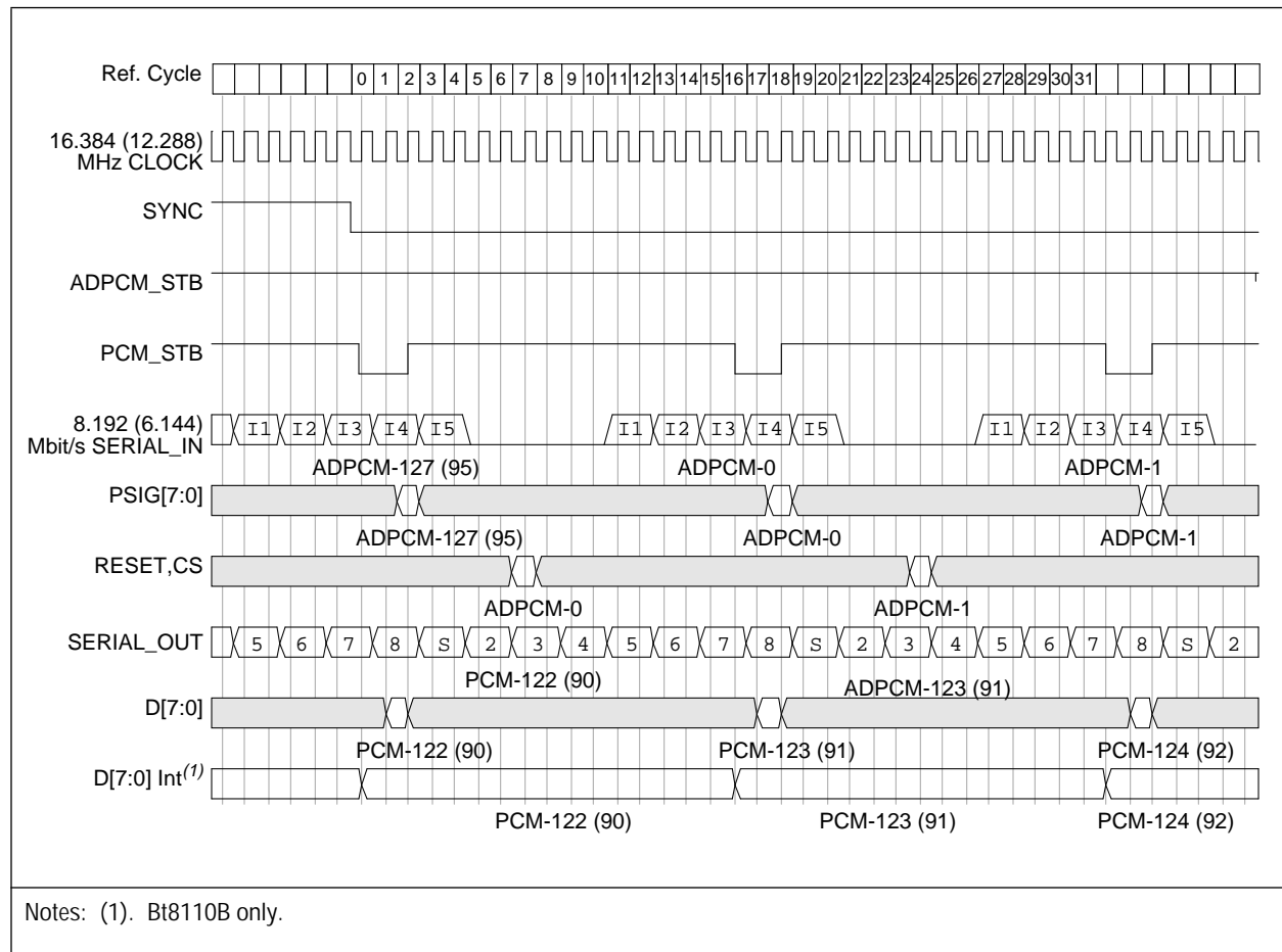
Figure A-4. 96- or 128-Channel Half-Duplex Decoder-Only Functional Timing
