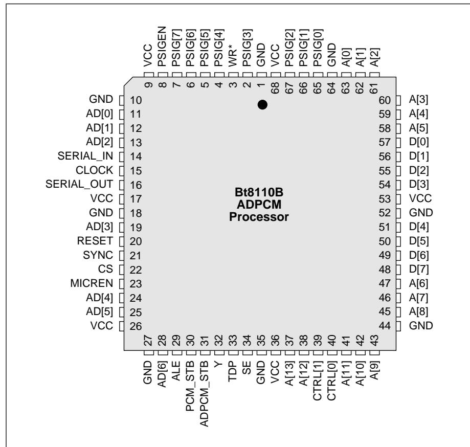
Figure 1-3. Bt8110B Pinout Diagram
