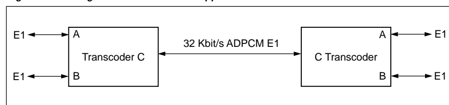
Figure E-2. Single-Board Transcoder Application
