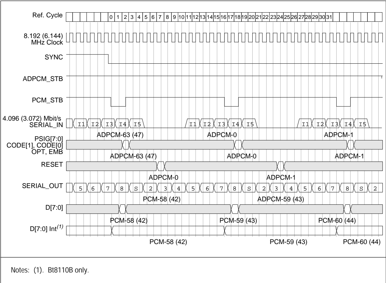
Figure 2-8. Hardware Control Decoder-Only Timing
