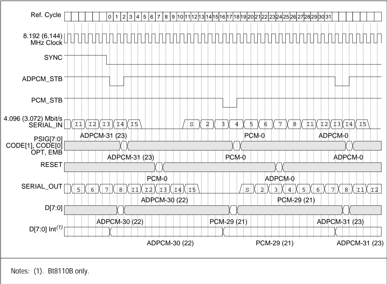
Figure 2-6. Hardware Control Interleaved Timing
