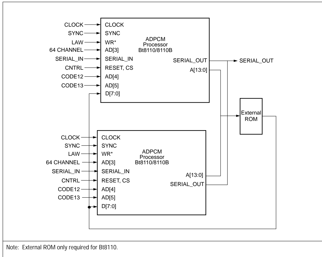
Figure A-1. 48- or 64-Channel Configuration of the Bt8110/8110B
