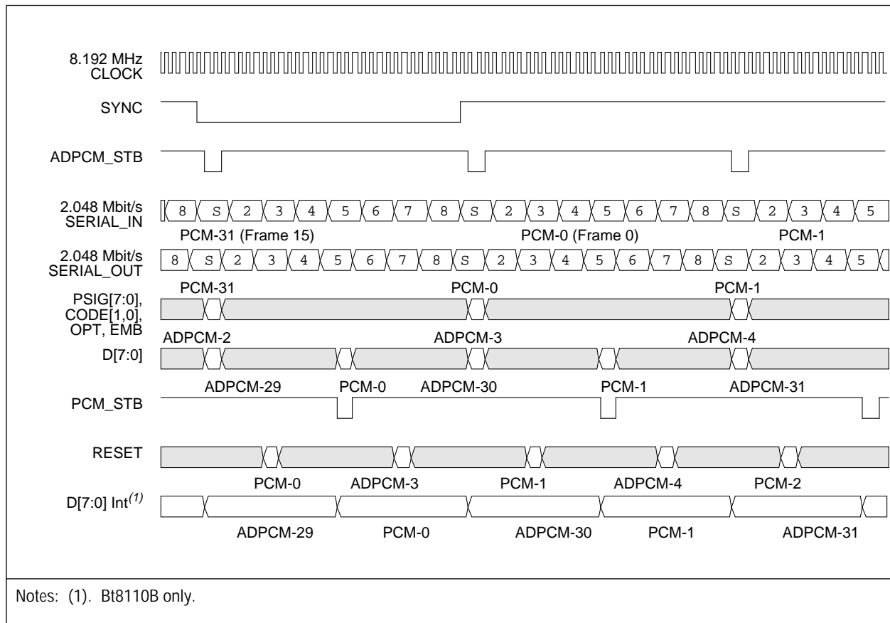
Figure C-2. E1 Speech Compression Functional Timing Diagram
