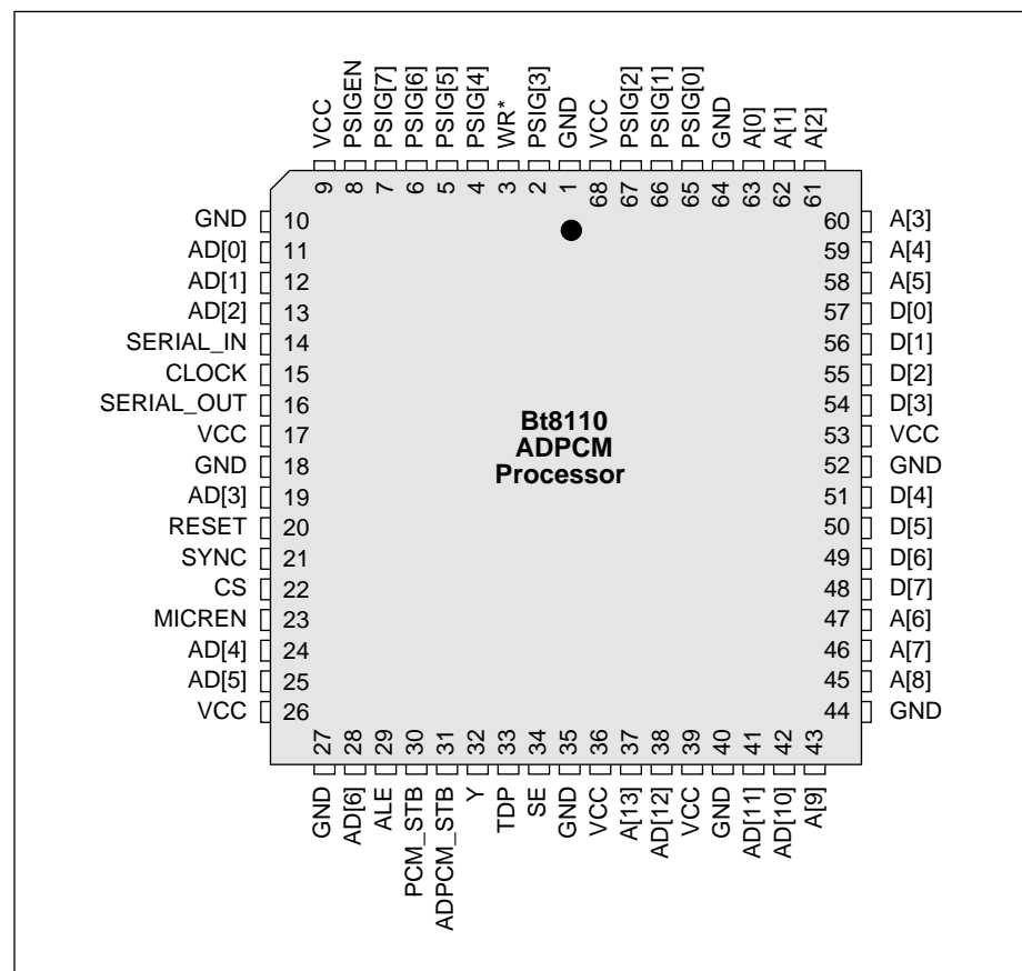
Figure 1-1. Bt8110 Pinout Diagram
