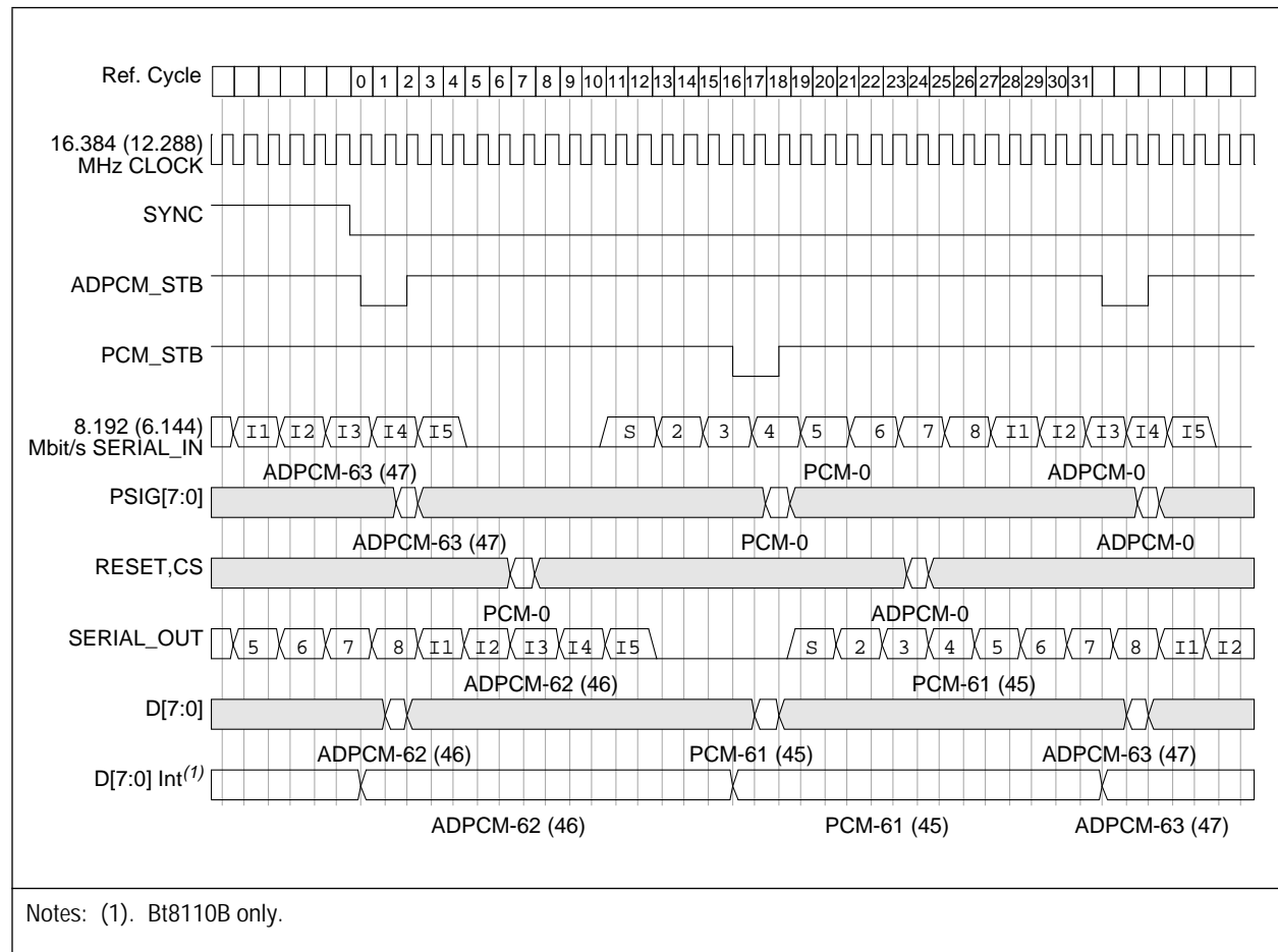
Figure A-2. 48- or 64-Channel Full-Duplex Interleaved Mode Functional Timing
