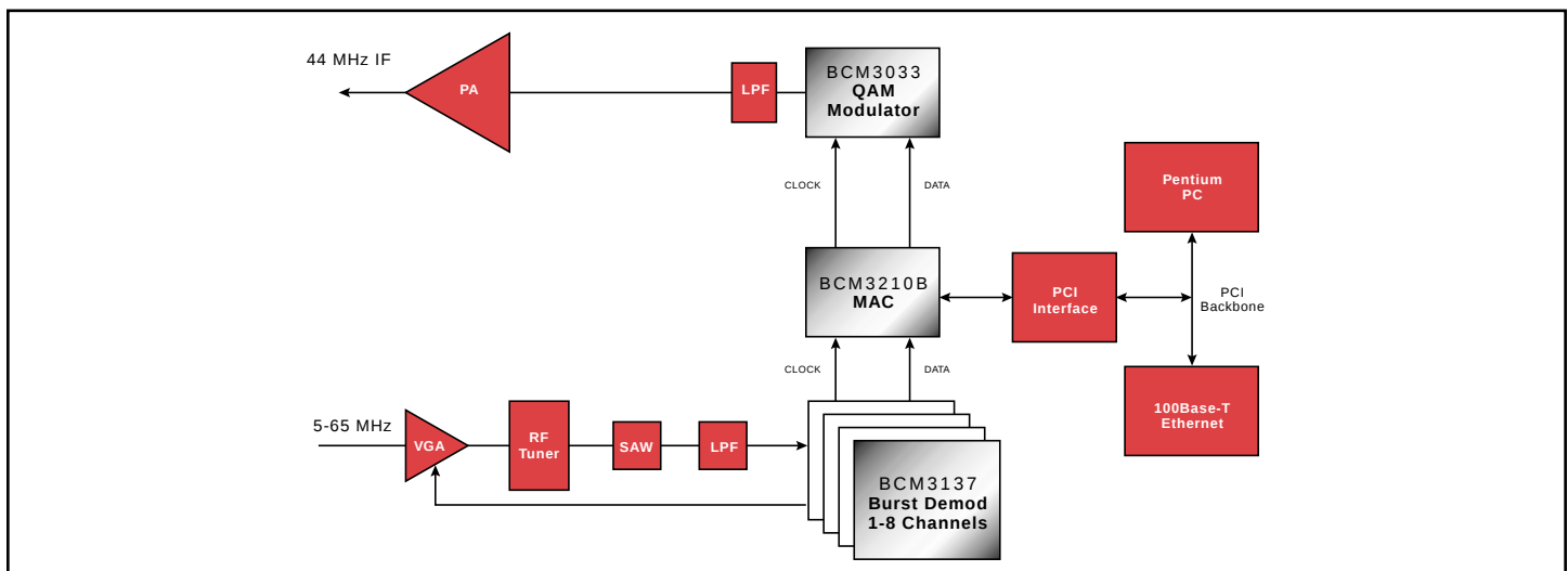
DOCSIS/EuroDOCSIS-compliant Cable Modem Termination System Block Diagram
