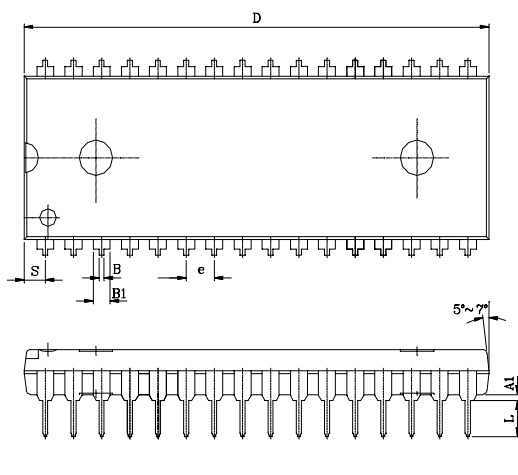
PDIP - 32
