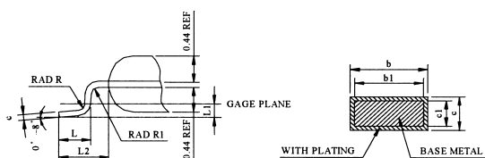
DETAIL "X"
