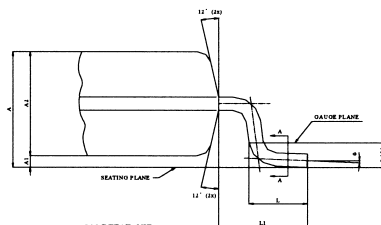
*A* DETAIL VIEW
